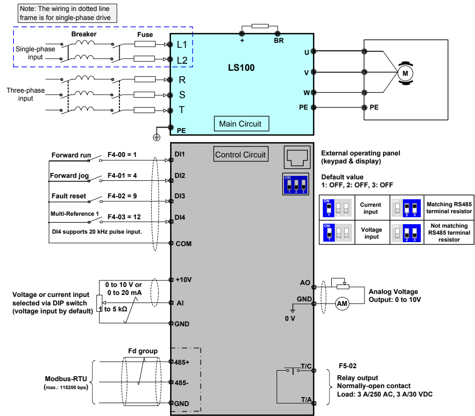
Figure 2-1 Single/Three-phase input terminal wiring (LS100S0.4B to LS100S2.2B, LS100T0.4B to LS100T3.7B)
